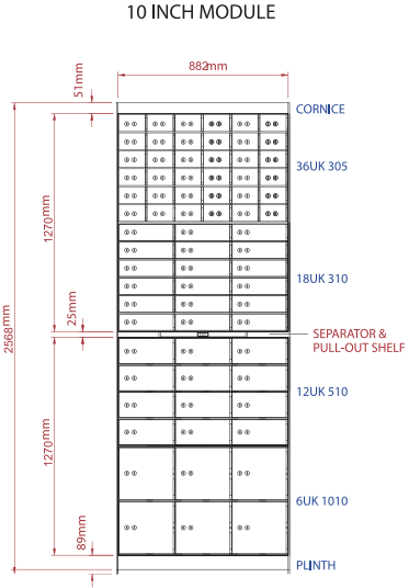
36UK 305 - 36 LOCKERS NETT WEIGHT : 183KG
